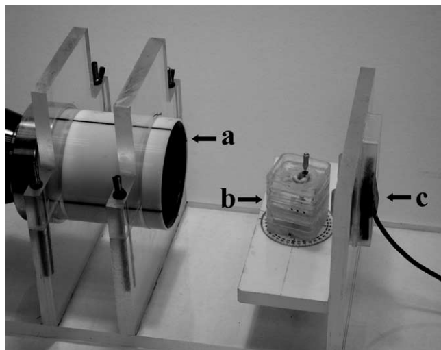
Figure 1. Plexiglass jig holding X-ray tube head (a), the turntable (b) containing the specimen, and the digital radiographic sensor (c).
